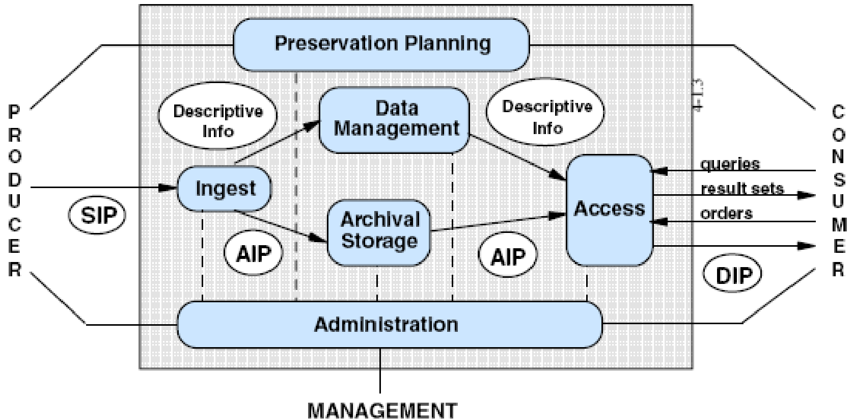
Figure 4-1: OAIS Functional Entities
